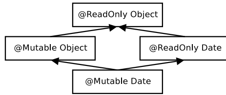
Figure 3: Type hierarchy for Javari’s ReadOnly type qualifier.
